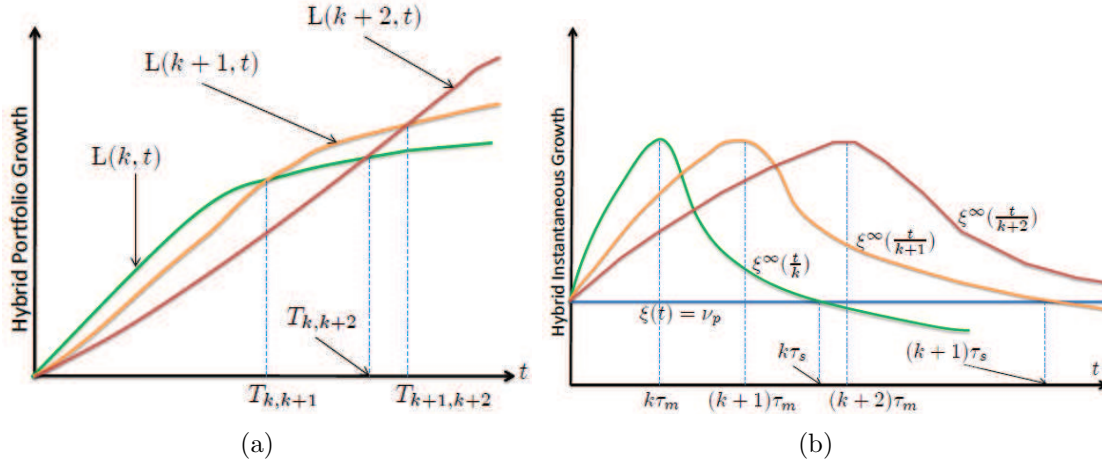
Figure 6.3 Illustrations of LURC, inflection point and EIPG of LURC.
