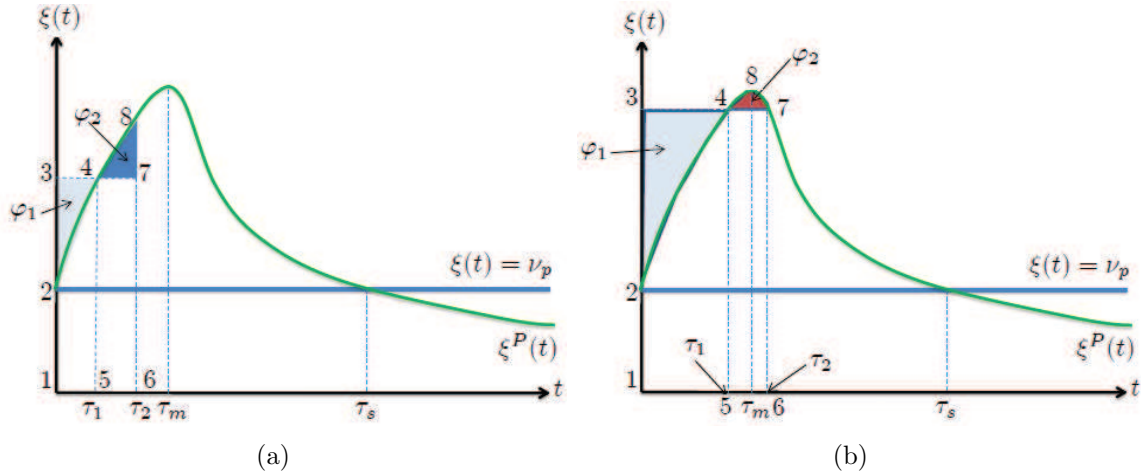
Figure 6.1 Two possible scenarios for deriving the lower bound for rebalance frequency.
