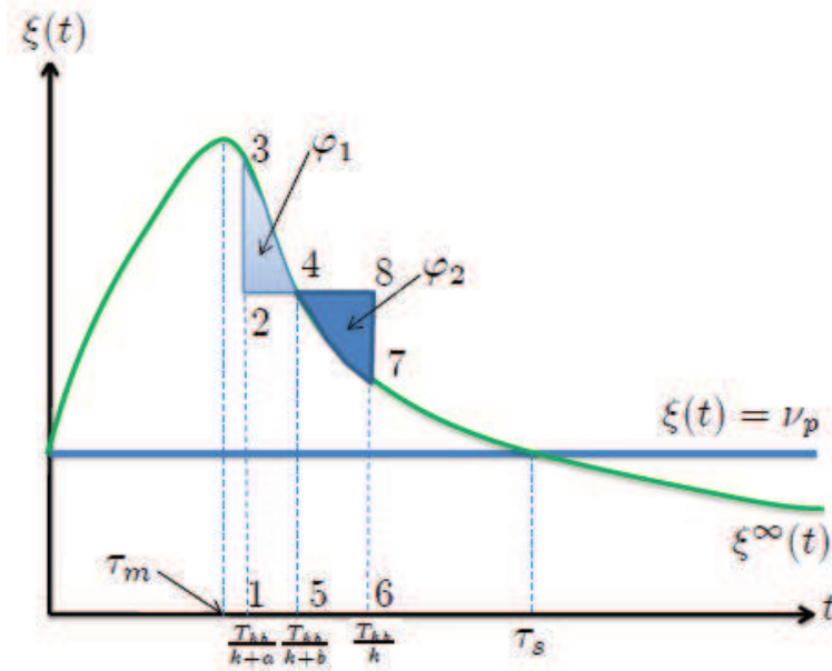
Figure 6.4 Illustration for proof of lemma 22.
